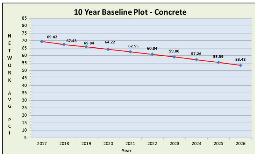
Figure 38: 10-Year "Do-Nothing" Baseline Plot for Concrete Roads
