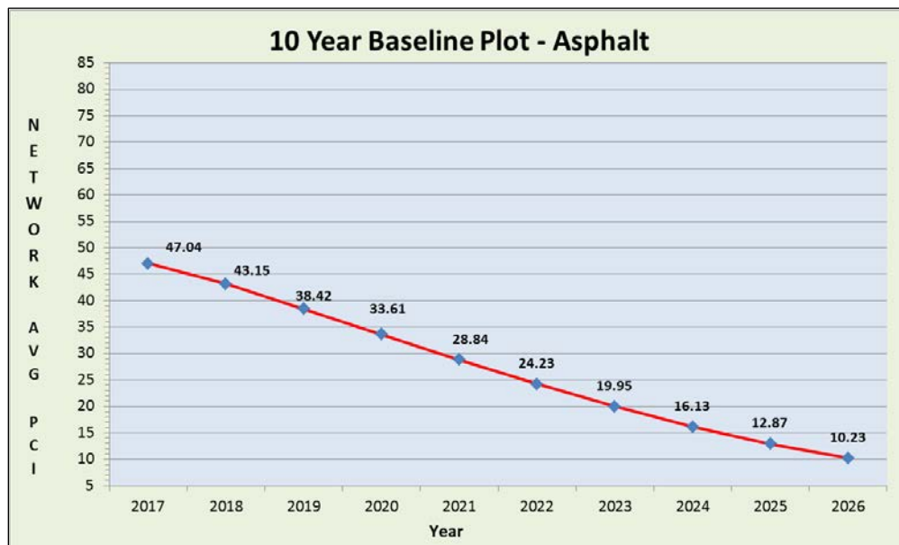
Figure 37: 10-Year "Do-Nothing" Baseline Plot for Asphalt Roads
