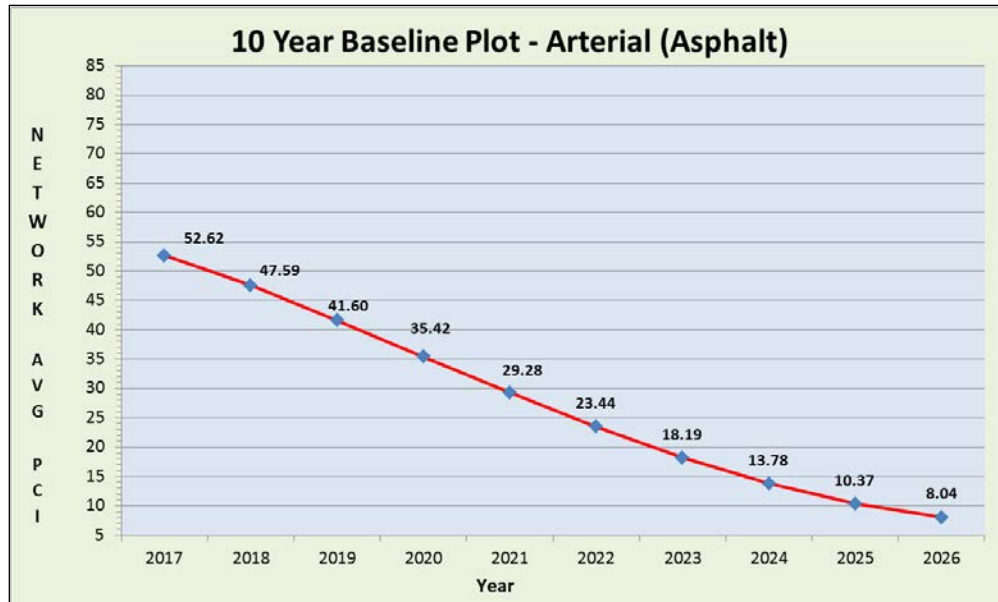
Figure 39: 10-Year “Do-Nothing” Baseline Plot for Arterial Asphalt Roads
