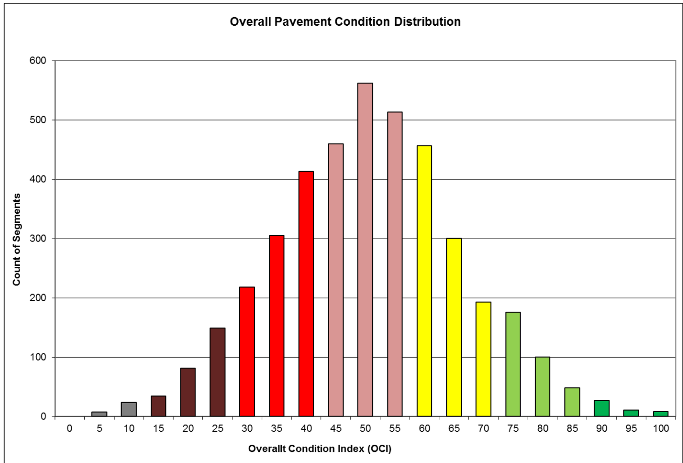
Figure 33: Salt Lake City, UT Overall Pavement Condition Distribution
