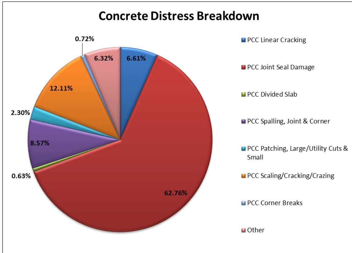
Figure 29: Salt Lake City, UT Concrete Distress Breakdown
