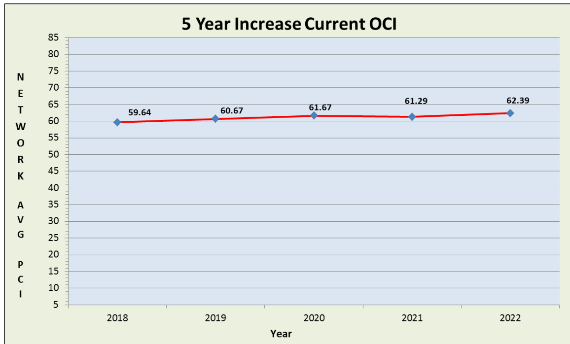
Figure 7: 5-Year Increase Current OCI Scenario – OCI Plot
