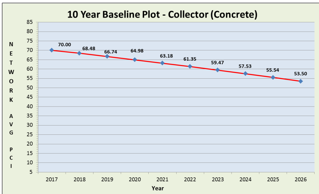
Figure 42: 10-Year “Do-Nothing” Baseline Plot for Collector Concrete Roads
