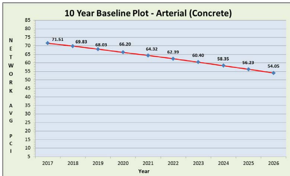
Figure 40: 10-Year “Do-Nothing” Baseline Plot for Arterial Concrete Roads
