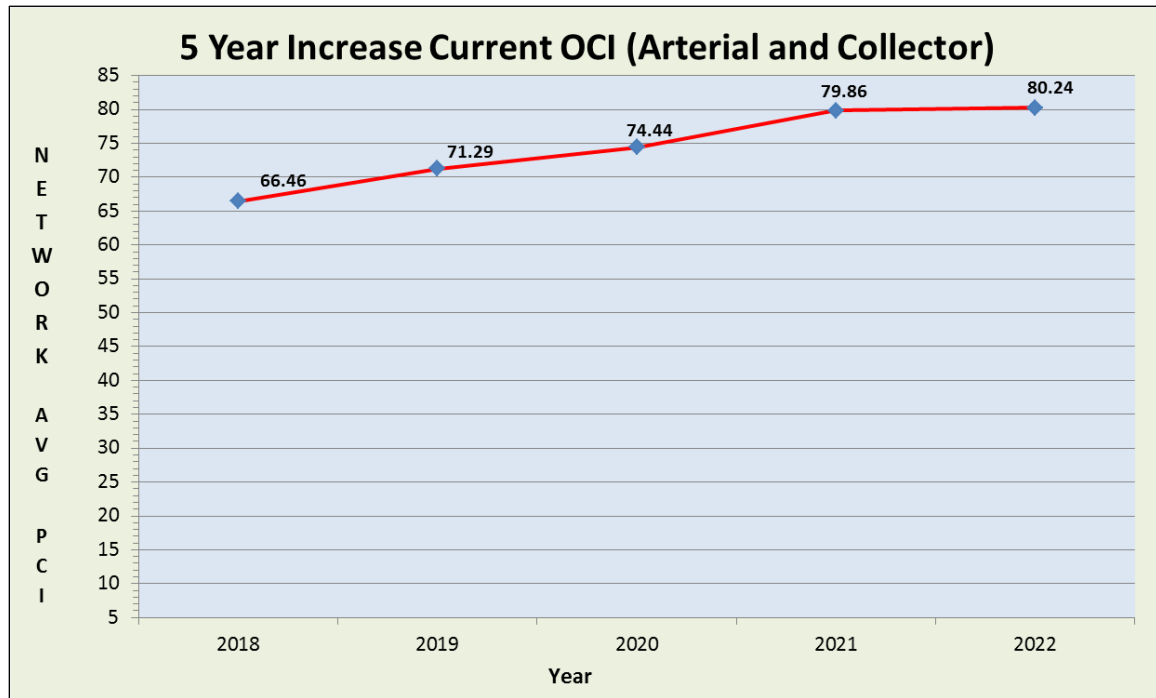
Figure 9: 5-Year Increase Current OCI Scenario (Arterial and Collector) – OCI Plot
