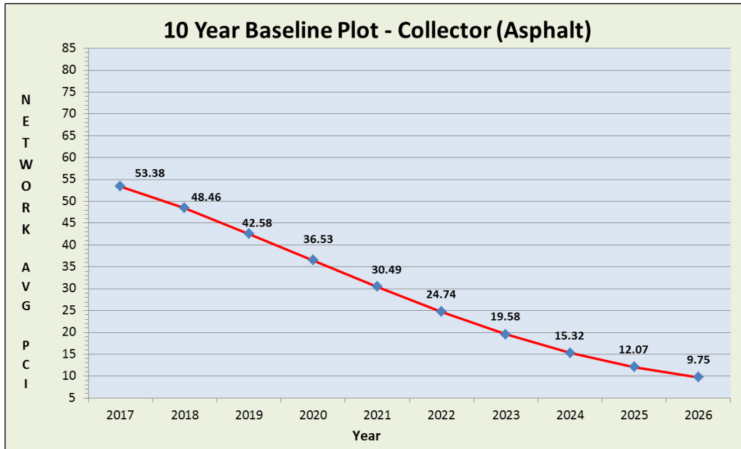
Figure 41: 10-Year “Do-Nothing” Baseline Plot for Collector Asphalt Roads
