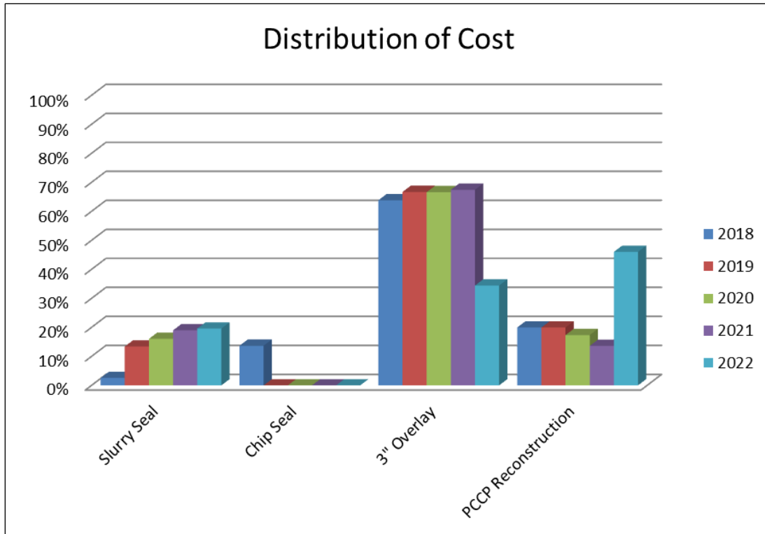
Figure 52: 5-Year Increase Current OCI Scenario – Distribution of Cost
