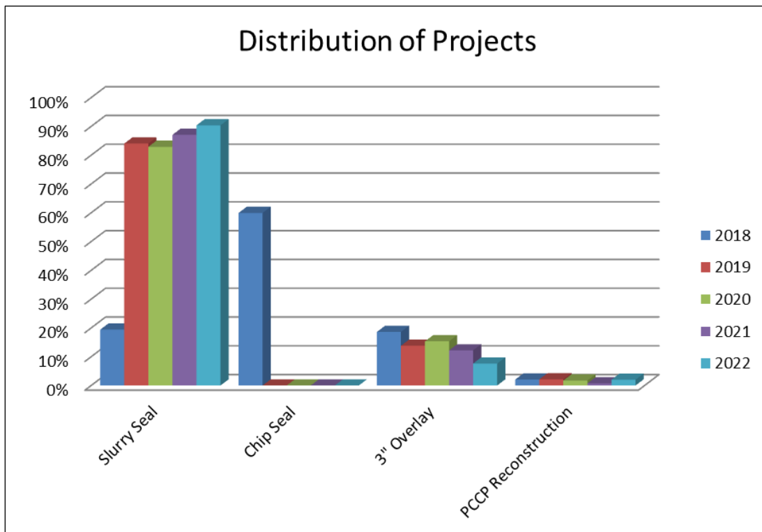
Figure 53: 5-Year Increase Current OCI Scenario – Distribution of Projects
