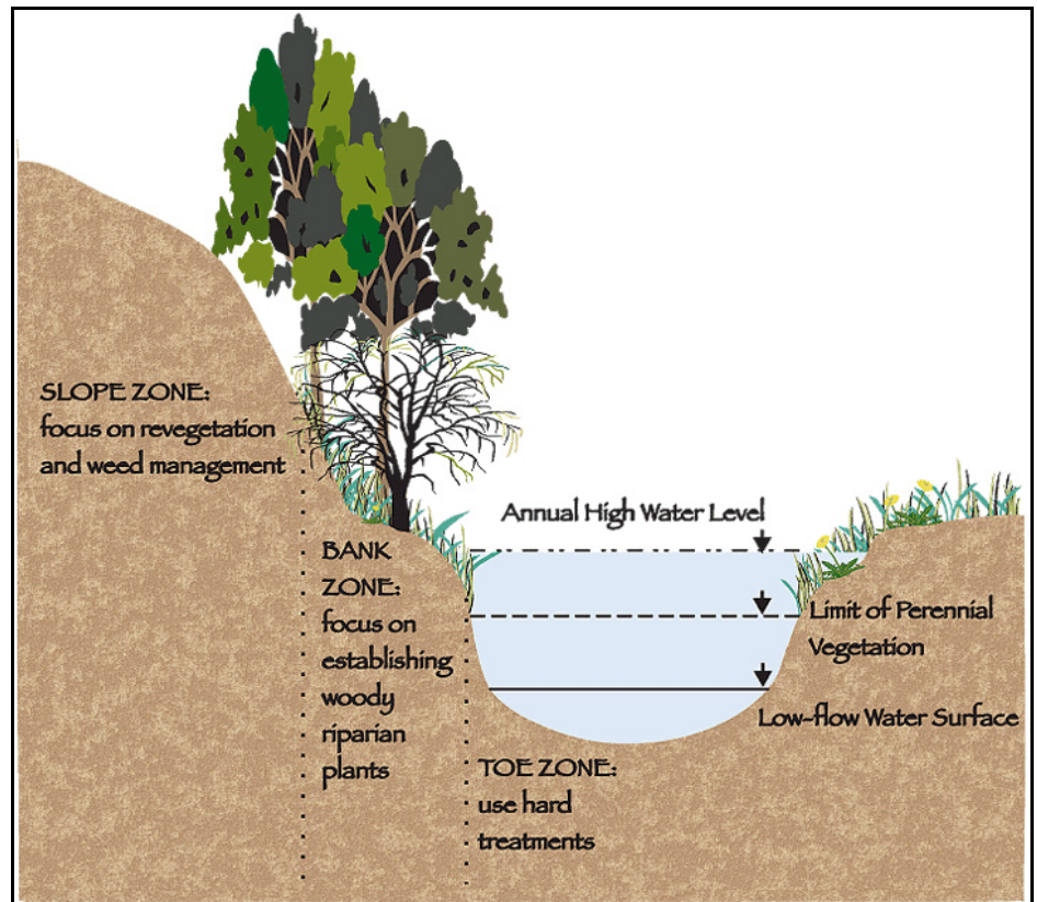
Figure 4.3. Schematic illustration of toe, bank, and upper slope zones and recommended treatment approaches.
