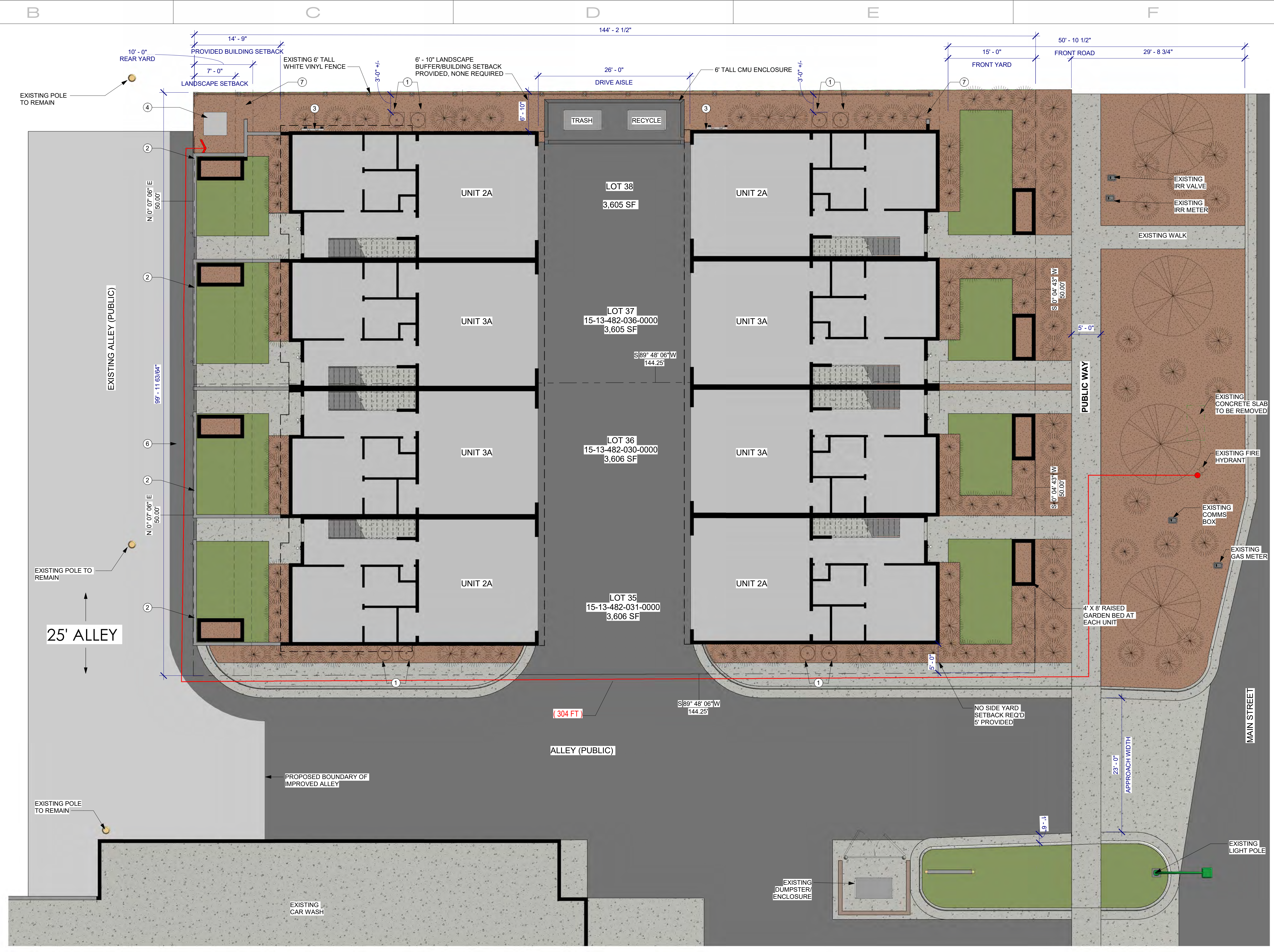
1 SITE PLAN A100 1/8" = 1'-0"
