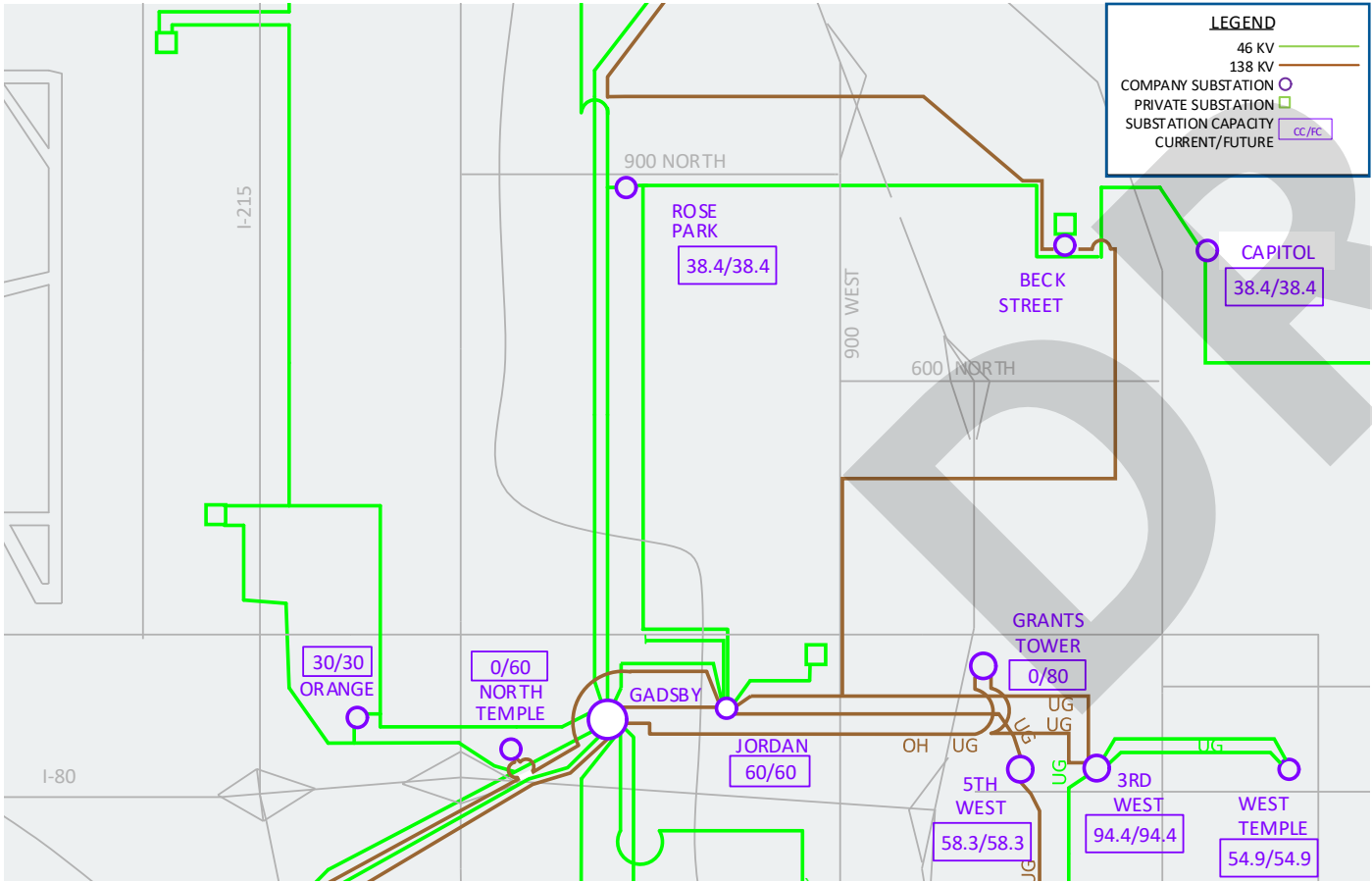
Northwest Salt Lake Area Transmission & Substation Plan
