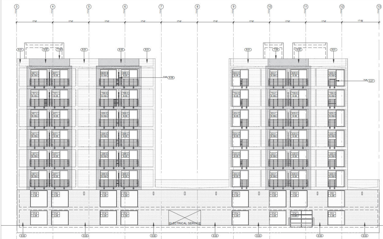
SOUTH ELEVATION
