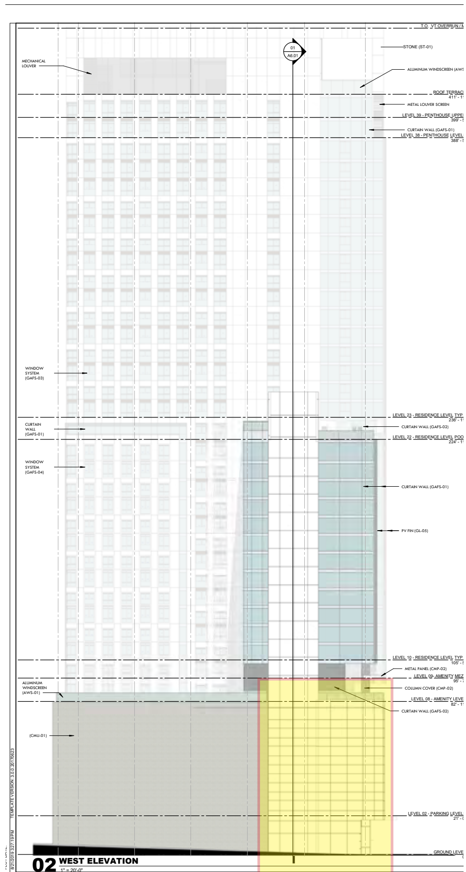
APPROVED DESIGN
