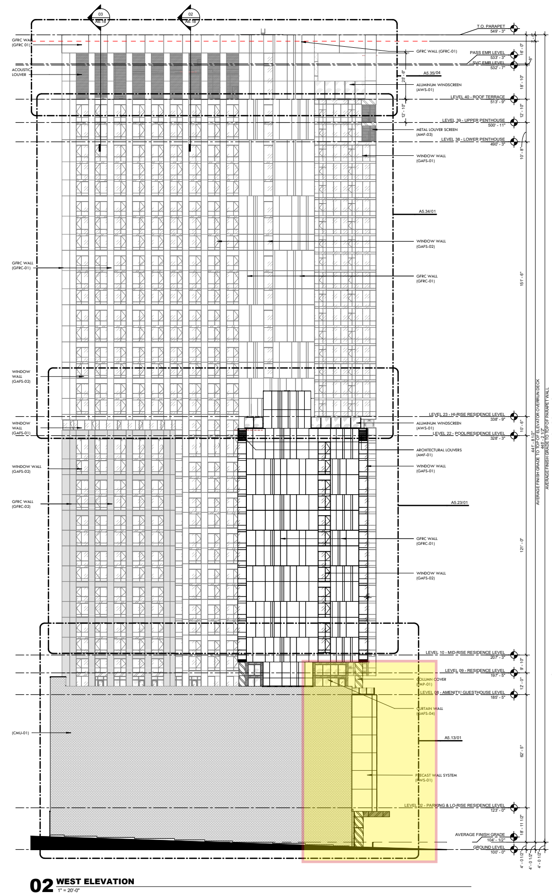
CURRENT DESIGN
