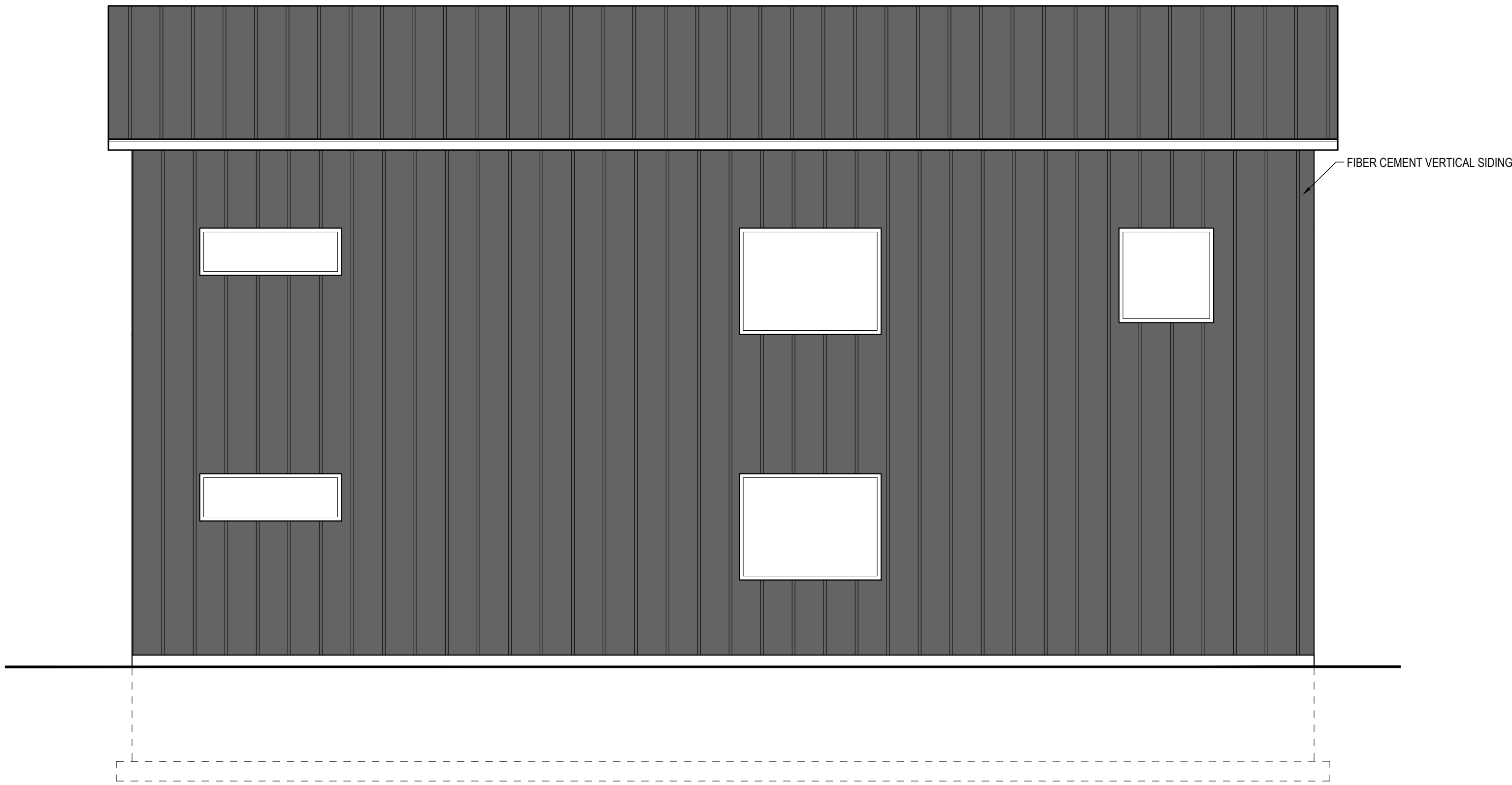
2 LEFT ELEVATION 1/8" = 1'-0" (ARCH B) 1/4" = 1'-0" (ARCH D)
