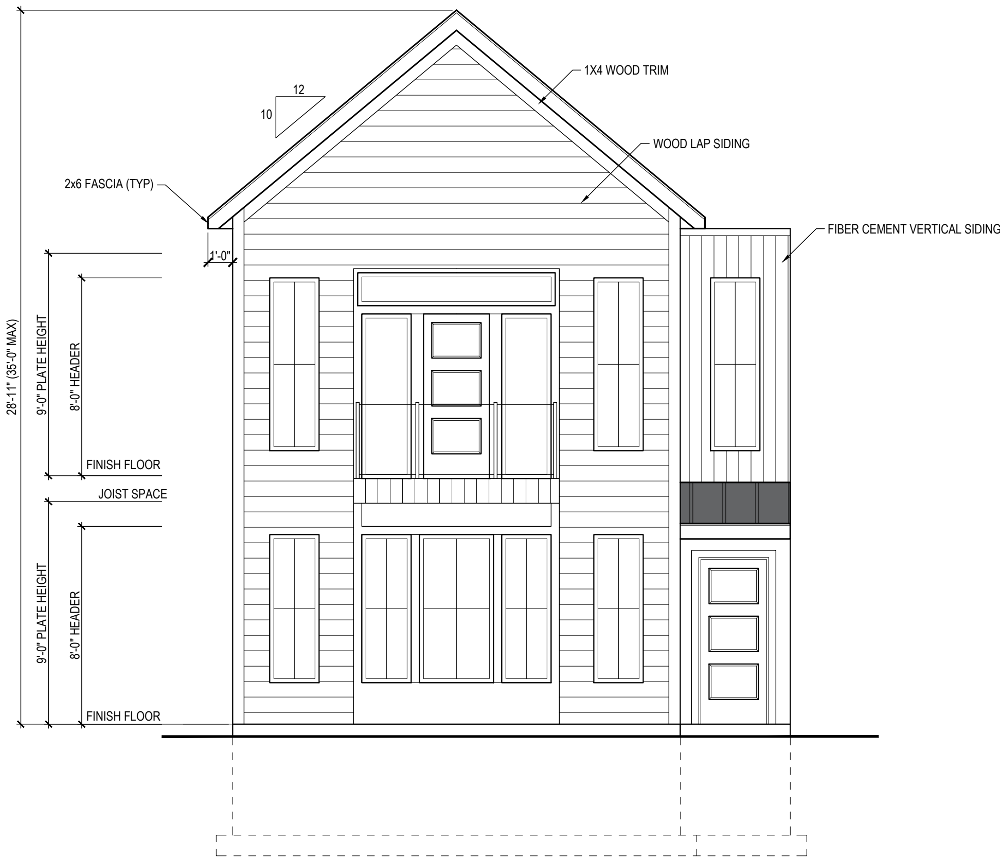
1 FRONT ELEVATION
