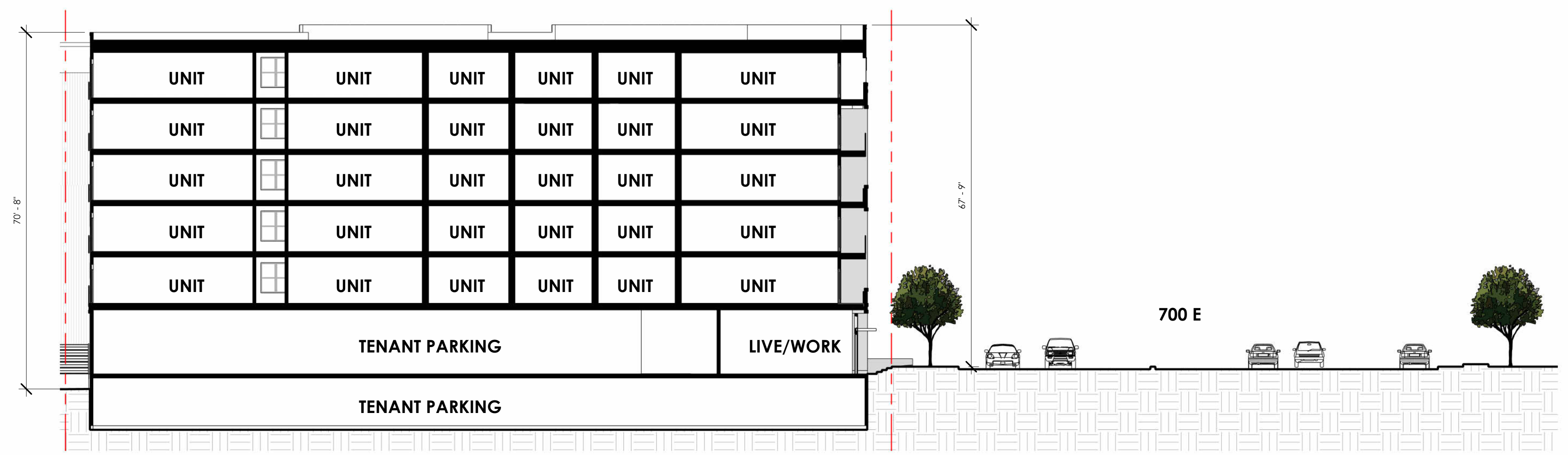
3 BUILDING SECTION 3 1/16" = 1'-0"
