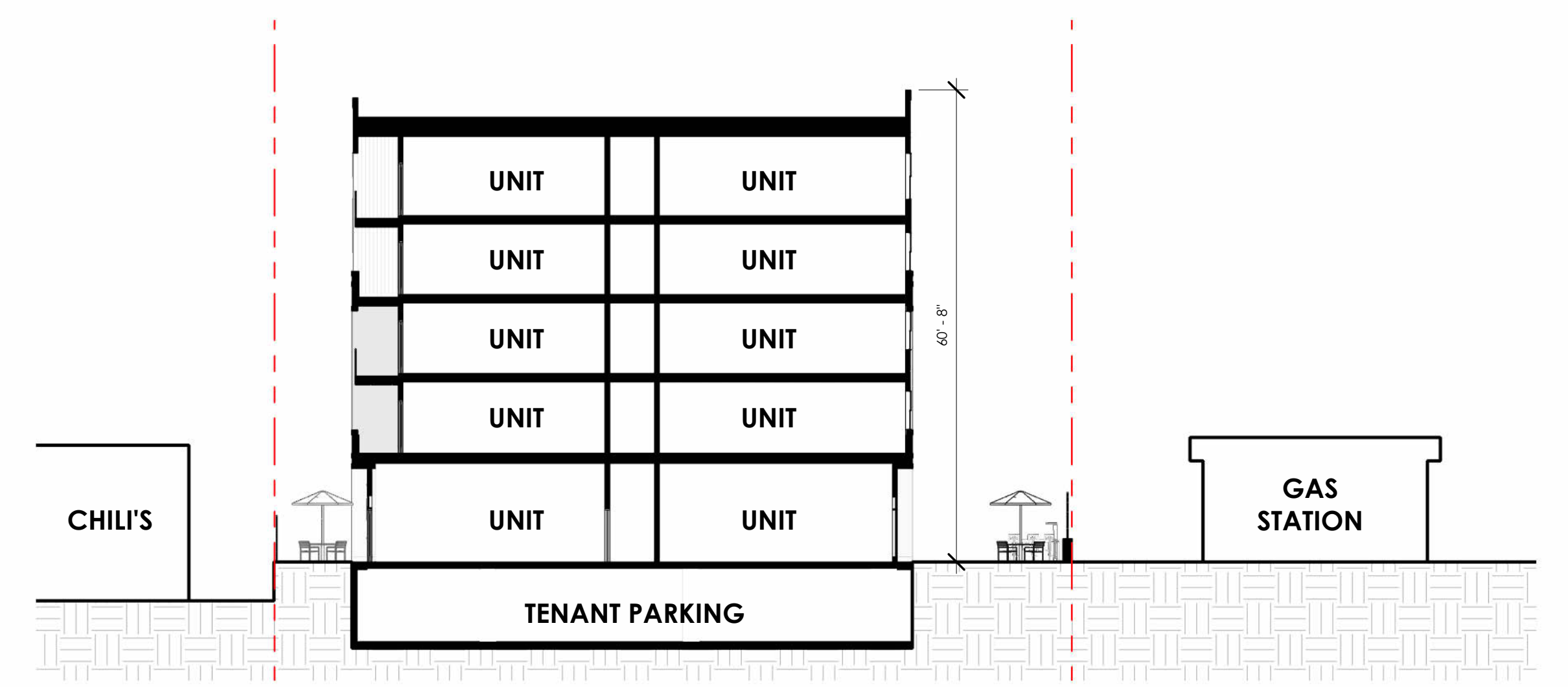
2 BUILDING SECTION 2 1/16" = 1'-0"
