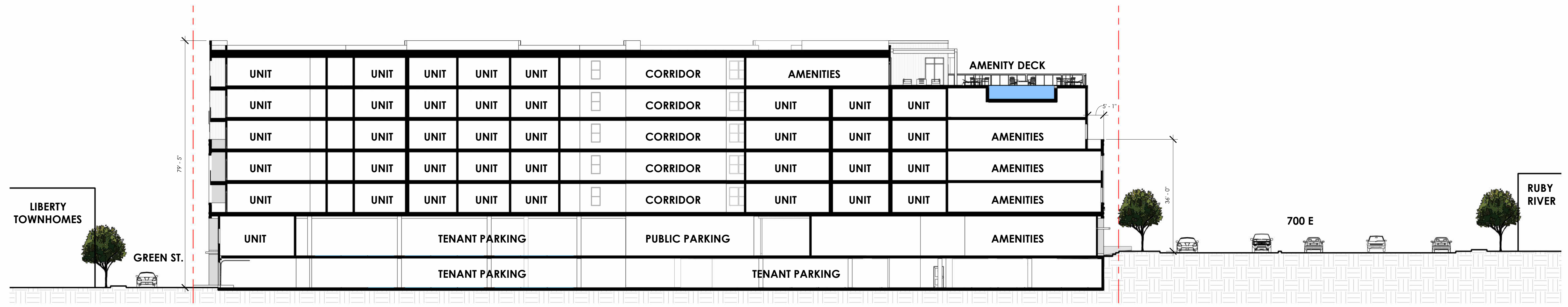
1 BUILDING SECTION 1 1/16" = 1'-0"
