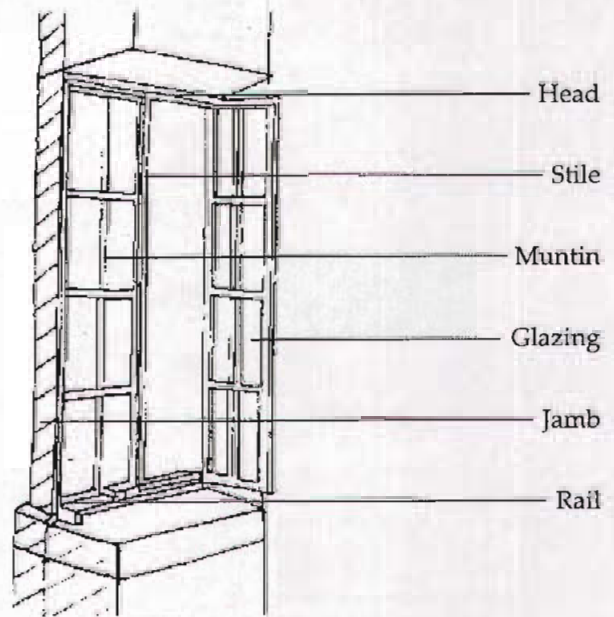
Casement window components
